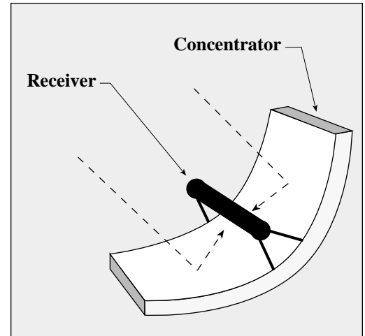
Fig. 1 A parabolic trough
