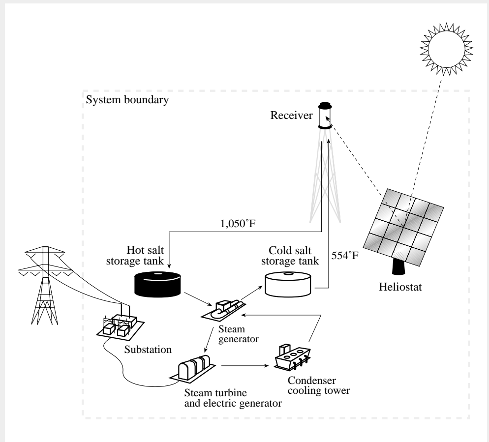
Fig. 3 Solar Two power tower system
